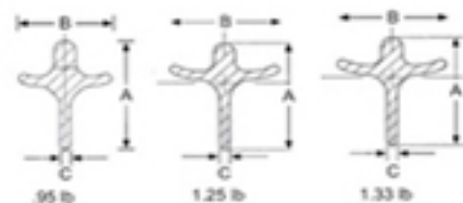
Studded T Post Raw Specification for silf fence
